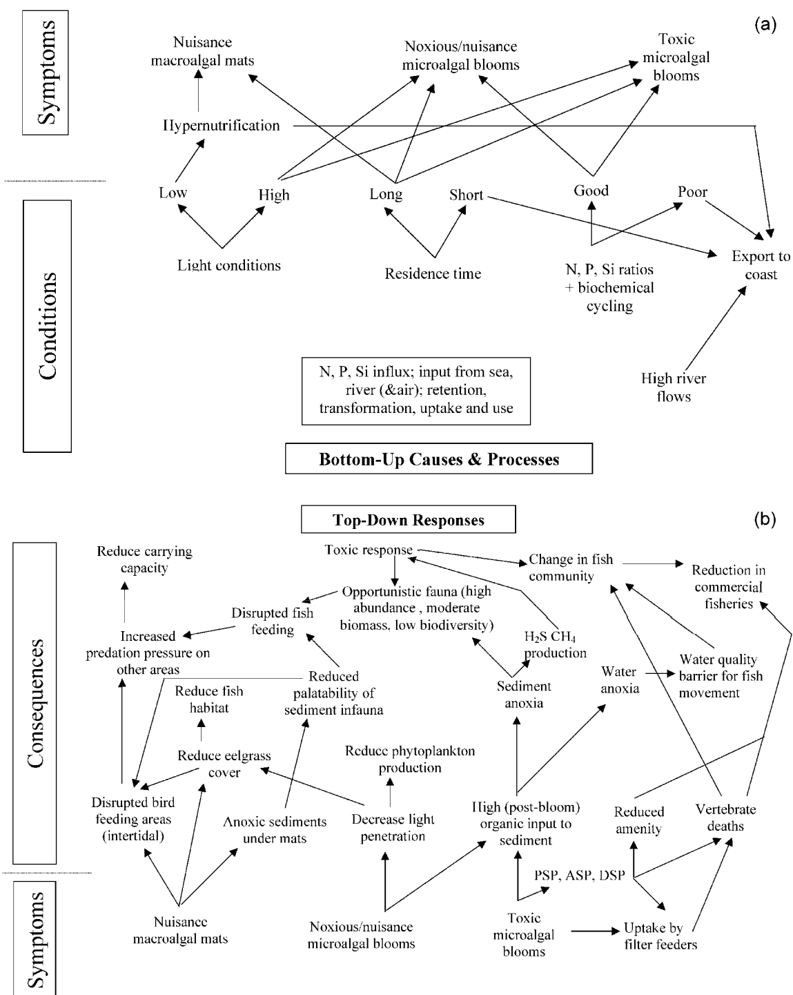
Figure 1. (a) Conceptual model – bottom-up causes and processes for nutrient effects. (b) Conceptual model – top-down responses for nutrient effects and eutrophication (adapted from Elliott & Hemingway, 2002).
