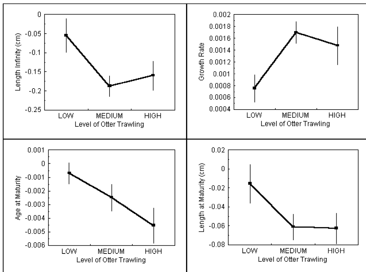
Figure 10.4.1.4.6 Variation in the regression coefficients ( \pm 1 S.E. of the coefficient) for the slopes of Length_{inf} , Growth Rate, Age_{Maturity} and Length_{Maturity} over the time period 1925 to 1995 in rectangles with different mean levels of annual international otter trawl effort over the period 1990 to 1995.
