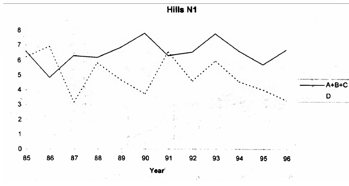
Figure 8.2.2.2.12 (The Barents Sea case study). Hills N1 calculated for 2 different areas in the Barents Sea. A+B+C is the western subarea while D is the eastern subarea.
