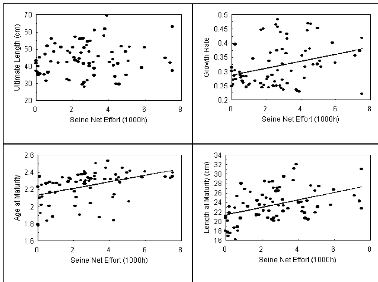
Figure 10.4.1.4.2. Relationship between Seine net effort in 75 ICES statistical rectangles and the average and Length_{infinite} , Growth Rate, Age_{Maturity} and Length_{Maturity} determined for 32 species making up >99% of the total number of individuals sampled in each rectangle.
