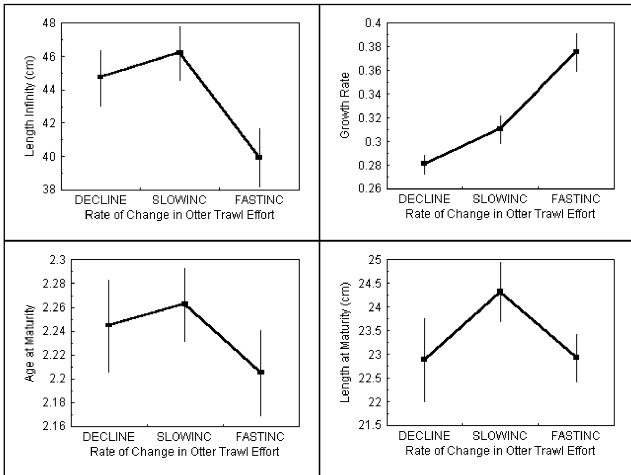
Figure 10.4.1.4.5. Variation in the mean ( \pm 1 \text{ S.E.} ) L_{inf} , Growth Rate, A_{mat} and L_{mat} determined for 32 species making up >99% of the total number of individuals sampled in each rectangle in groups of rectangles with different annual rates of change in otter trawl effort.
