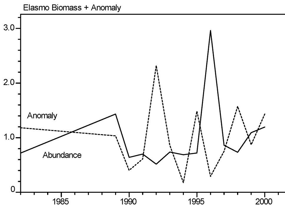
Figure 10.4.3.4.3.6 Elasmobranch abundance and anomaly of the centre of mass.
