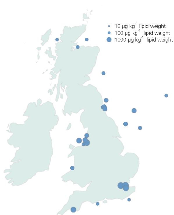
Figure 4.27 Median concentrations of the sum of the ICES 7 CBs in fish liver ( \mu\text{g kg}^{-1} lipid weight)
