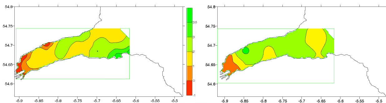
Figure 93. (a) 1976 \text{Log}_{10} crustacean abundance (Based on 42 sites) and (b) 2001 \text{Log}_{10} crustacean abundance (based on 20 sites) (Azoic sites plotted as -1)
