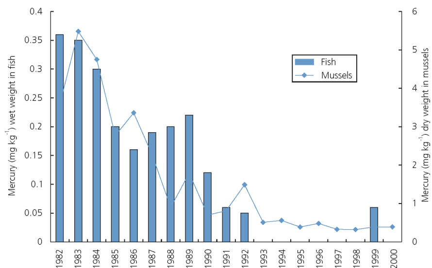
Figure 23. Mercury in fish and mussels in the Forth estuary
