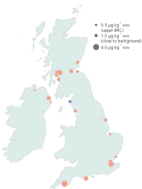
Figure 4.20. Median concentrations of CB 153 in mussels (µg kg -1 wet weight) and their relationship to BRCs
