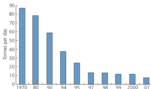
Figure 74. Average daily load of ammonia released to the estuary between 1970 and 2001
