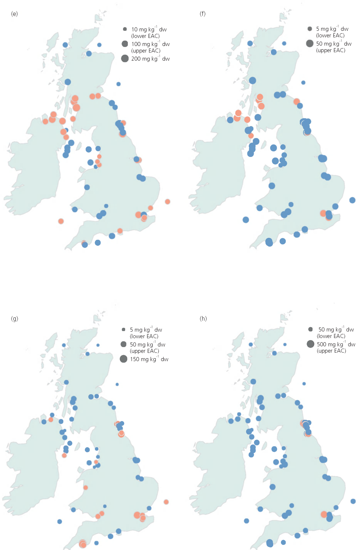
Figure 4.11. continued: Median concentrations of (e) chromium, (f) nickel, (g) copper and (h) zinc in sediments, relative to their EACs
