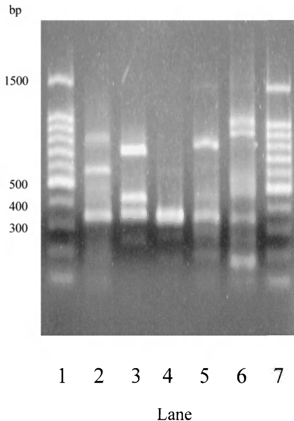
Figure 2. Amplification of the internal sequences by PCR with ODH-9F and ODH-11R in various marine invertebrates. Lanes 1 and 7, 100-bp DNA ladder; lane 2, Arabella iricolor ; lane 3, Haliotis discus hannai ; lane 4, Patinopecten yessoensis ; lane 5, Spisula sachalinensis ; lane 6, Meretrix lusoria . The arrow indicates target fragments.
