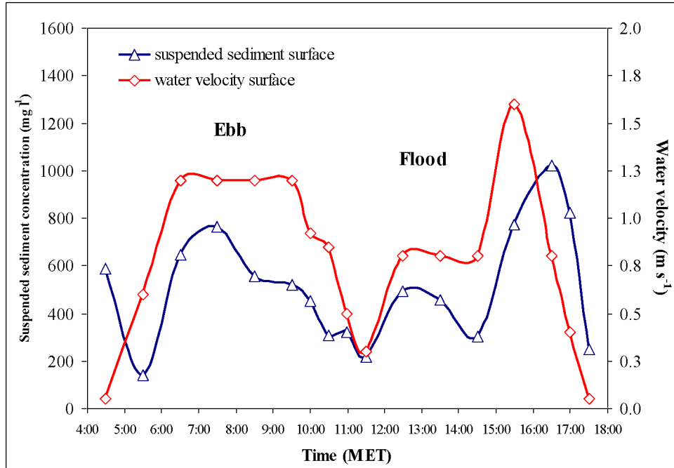
Figure 5.8. Suspended sediment concentration and water velocity at near surface layer during the full tide-cycle measurements at Kruikebe on May 19, 2011.
