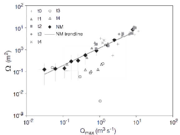
Fig. 9. Maximum tidal discharge Q_{max} versus cross-sectional area \Omega . Grey symbols represent the ditch cross-sections of the CRT marsh, white symbols the cross-sections of the newly formed channels in the CRT marsh. NM=the natural marsh.
