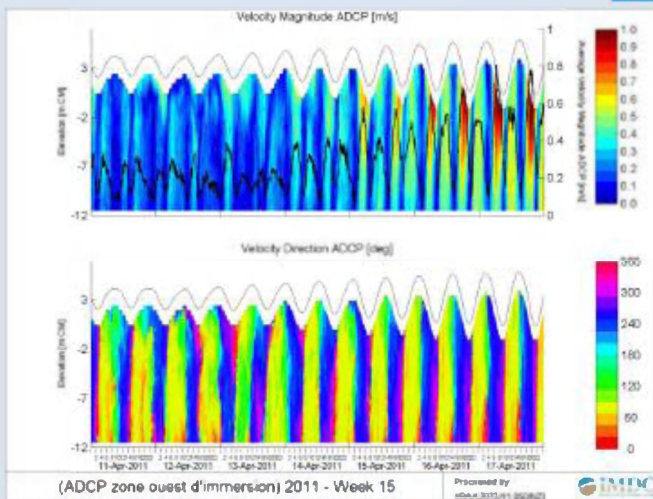
Bottom fixed current measurements at La Lamberde (La lamberde, 2011)
