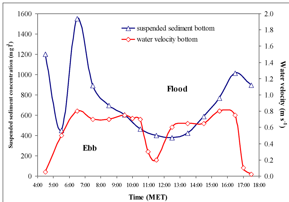
Figure 5.9. . Suspended sediment concentration and water velocity at near bottom layer during the full tide-cycle measurements at Kruikebe on May 19, 2011.
