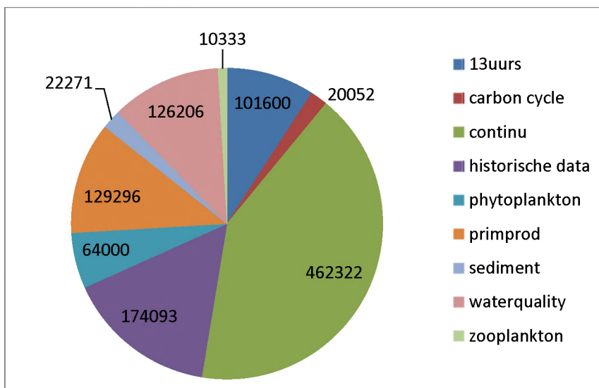
Figure 9.1. Verdeling datatypes
