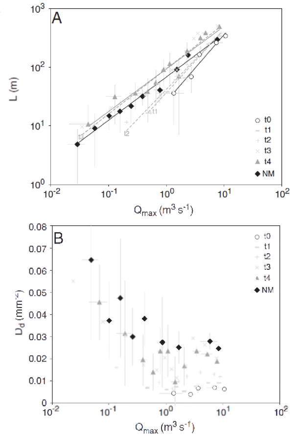
Fig. 8. (A) Relationship between maximum tidal discharge Q_{max} and mainstream length L , NM in legend=natural tidal marsh. (B) Relationship between maximum tidal discharge Q_{max} and Hortonian drainage density D_d .
