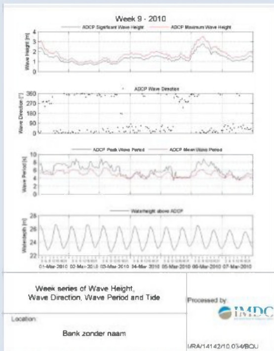
Bottom fixed wave measurements at North Sea (Eidepasco, 2010)
