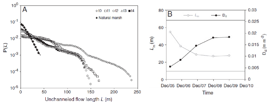
Fig. 5. (A) Probability density function of the unchanneled flow length L (i.e., the distance of any platform location to the nearest channel), for t0 up to t4 at the constructed CRT marsh, and for the natural tidal marsh (NM). Linear trends on the semi-logarithmic plots are presented for the CRT marsh at t0, and for the natural tidal marsh. (B) Evolution of the mean unchanneled flow length L_m and the Hortonian drainage density D_d in the CRT marsh. Horizontal lines represent the mean unchanneled flow length (grey line at 8.9 m) and the Hortonian drainage density (black line at 0.0256 m m -2 ) for the natural tidal marsh.
