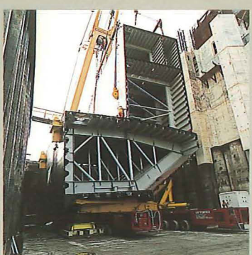
Deurcompartiment
