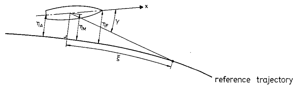
Figure 3 Track keeping autopilot (1) : conventions
