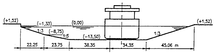
Figure 2 Canal Terneuzen - Ghent : standard cross-section ([1], [2])
