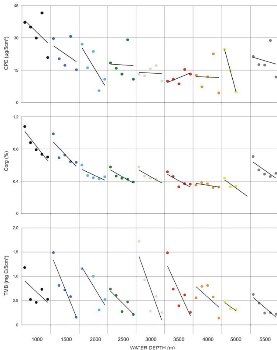
Figure 8. The temporal development of concentrations in chloroplastic pigment equivalents, (CPE), organic carbon ( C_{org} ), and total microbial biomass (TMB) in sediments along the HAUSGARTEN depth transect between 2000 and 2004 showed generally decreasing values.
