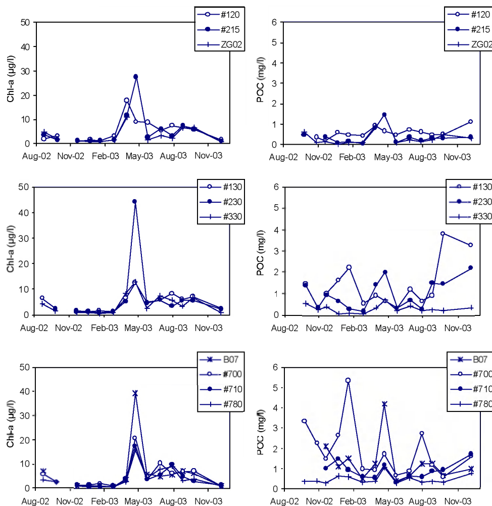
Fig. 2. Seasonal trend in the chlorophyll a and the POC concentrations for the ten stations investigated. The stations are grouped per transect: on the Nieuwpoort transect stations 120, 215 and ZG02, on the Oostende transect stations 130, 230 and 330 and on the Scheldt transect stations B07, 700, 710 and 780.
