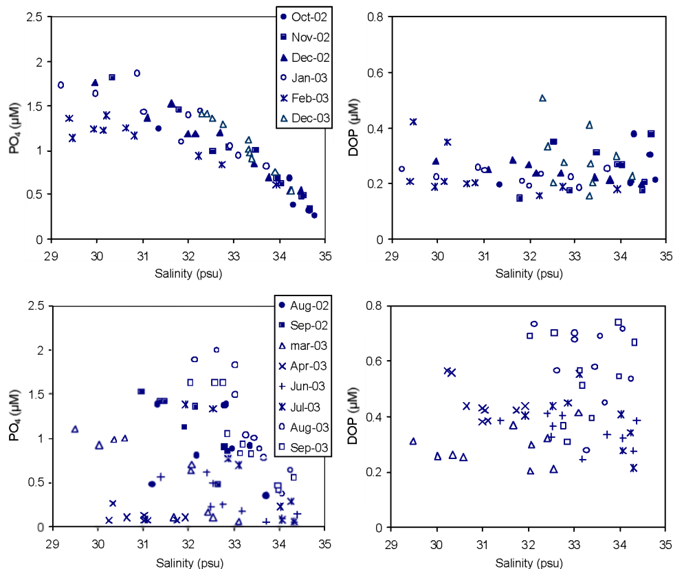
Fig. 10. PO 4 and DOP concentrations versus salinity, data of all the stations in different months. For the month of May, no salinity data were available. DOP was not determined for the months of August and September 2002.
