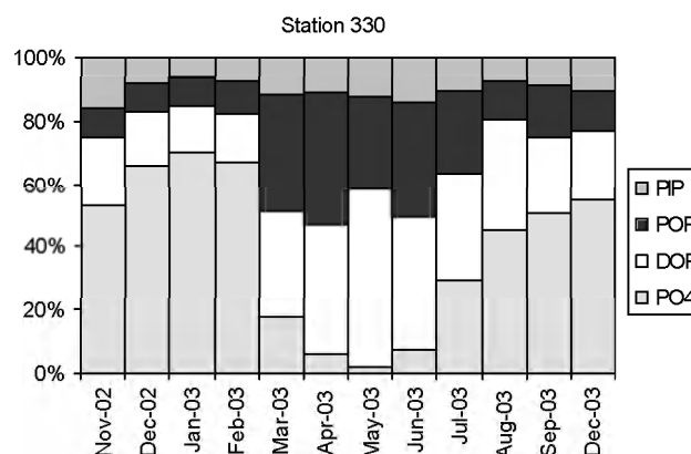
Fig. 9. Relative contributions of \text{PO}_4 , DOP, POP and PIP to the total P for station 330.
